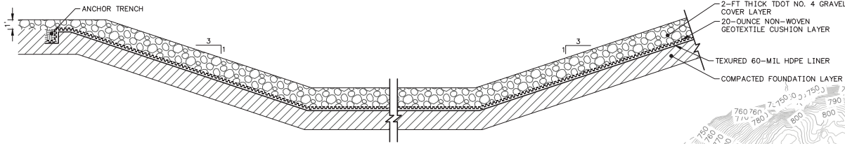
(A) SECTION (TYP) STORMWATER POND (NOTE 4) SCALE: N.T.S. XREF: 50772098
