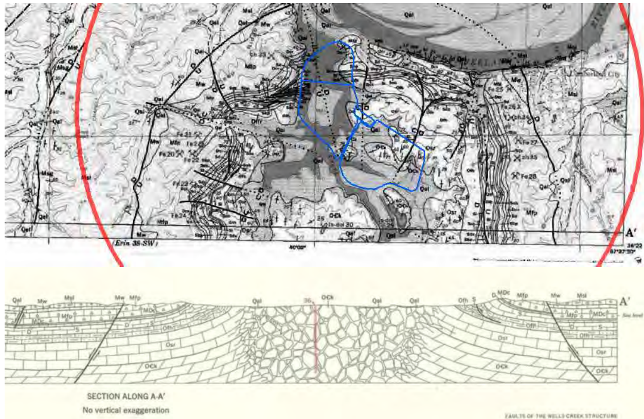
Figure 2. Excerpt from the geologic map of the Cumberland City Quadrangle, Tennessee for the Cumberland Fossil Plant study area (red) (Tiedemann et al., 1968).
